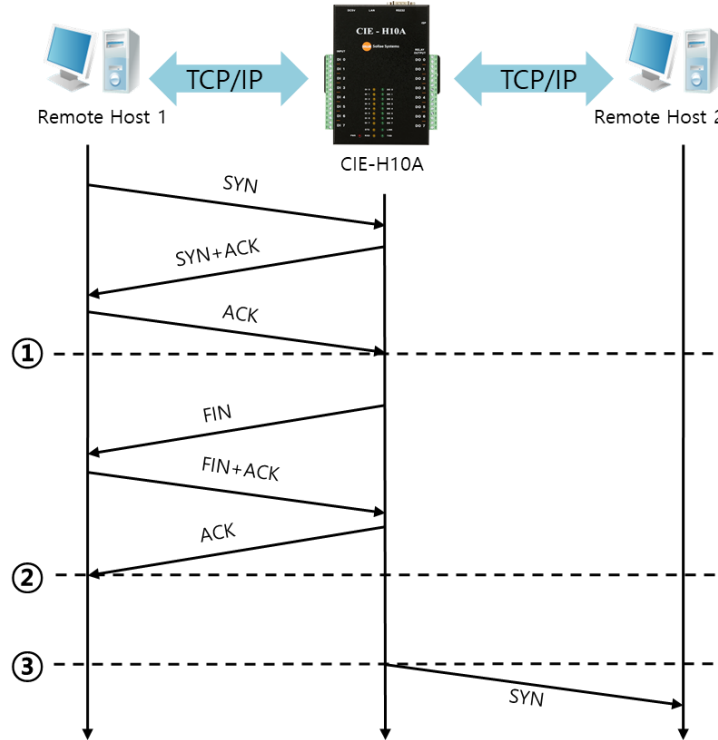
Fig 6-4 time chart for activating [TCP Server] option
