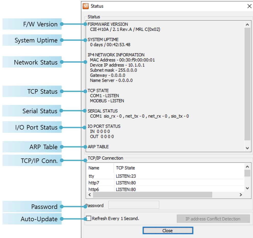
Figure 7-13 status window of ezManager
