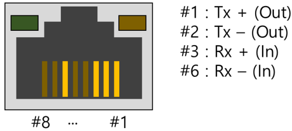
Figure 1-10 the RJ45 connector
