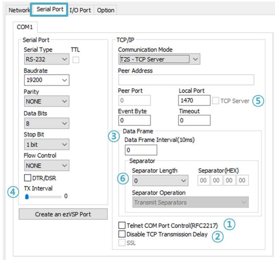
Figure 8-5 Serial Port Tab
