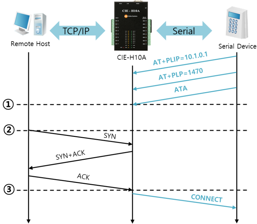
Figure 6-5 a passive TCP connection
