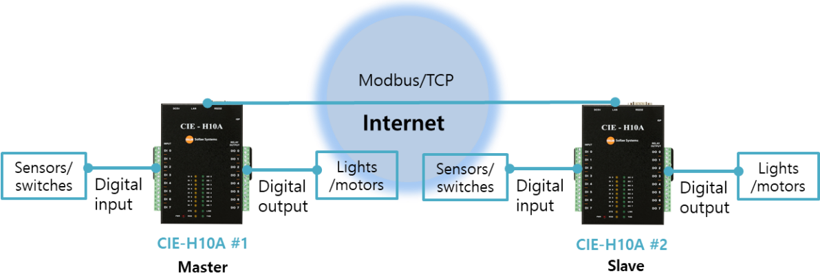
Figure 1-3 internet switch
