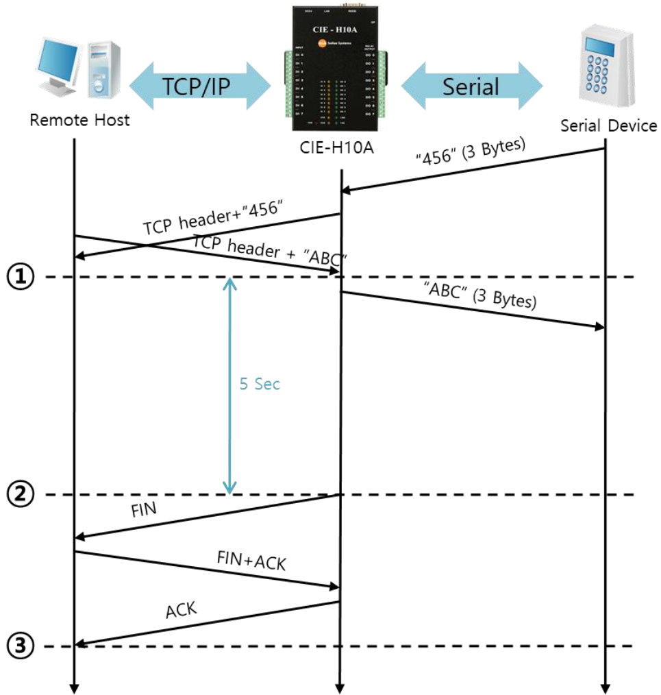
Figure 6-3 time chart
