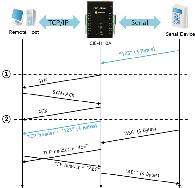
Figure 6-5 time chart
