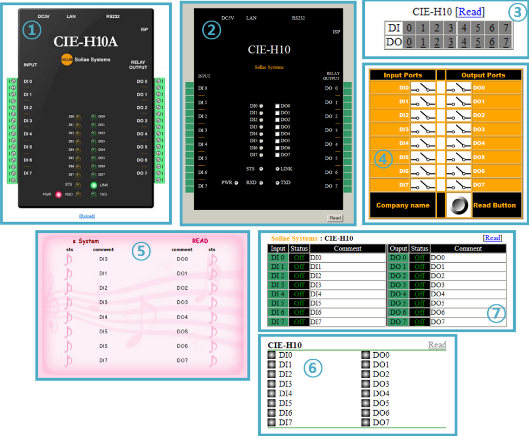
Figure 5-3 examples of web page
