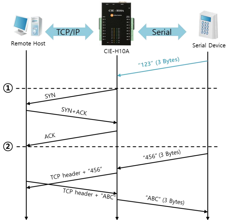
Figure 6-4 time chart
