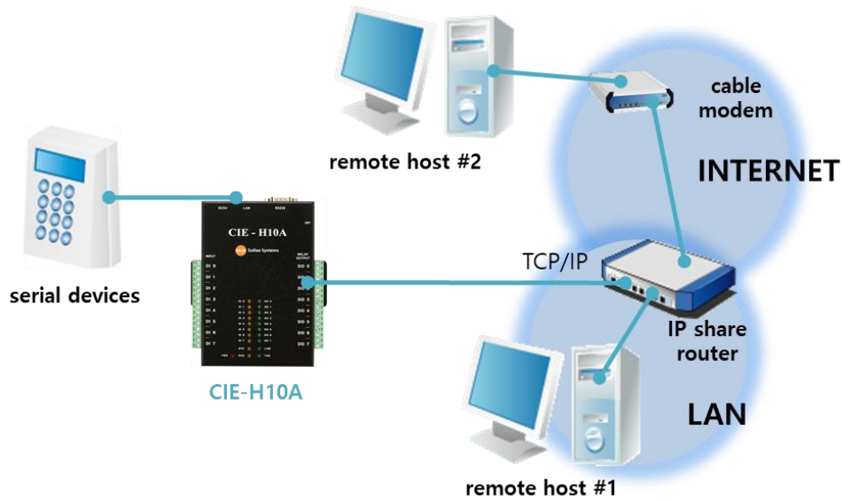
Figure 1-6 serial device server
