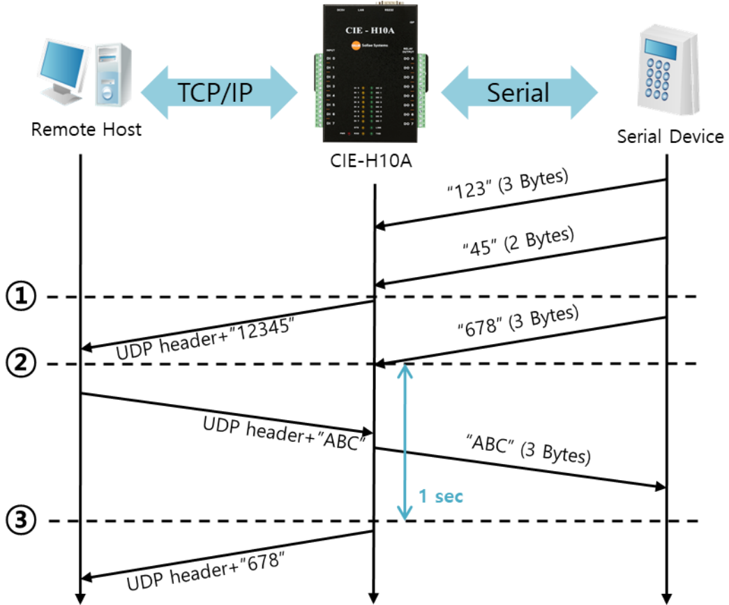
Figure 6-7 time chart for block size is 5 bytes and Data Frame Interval is 1s
