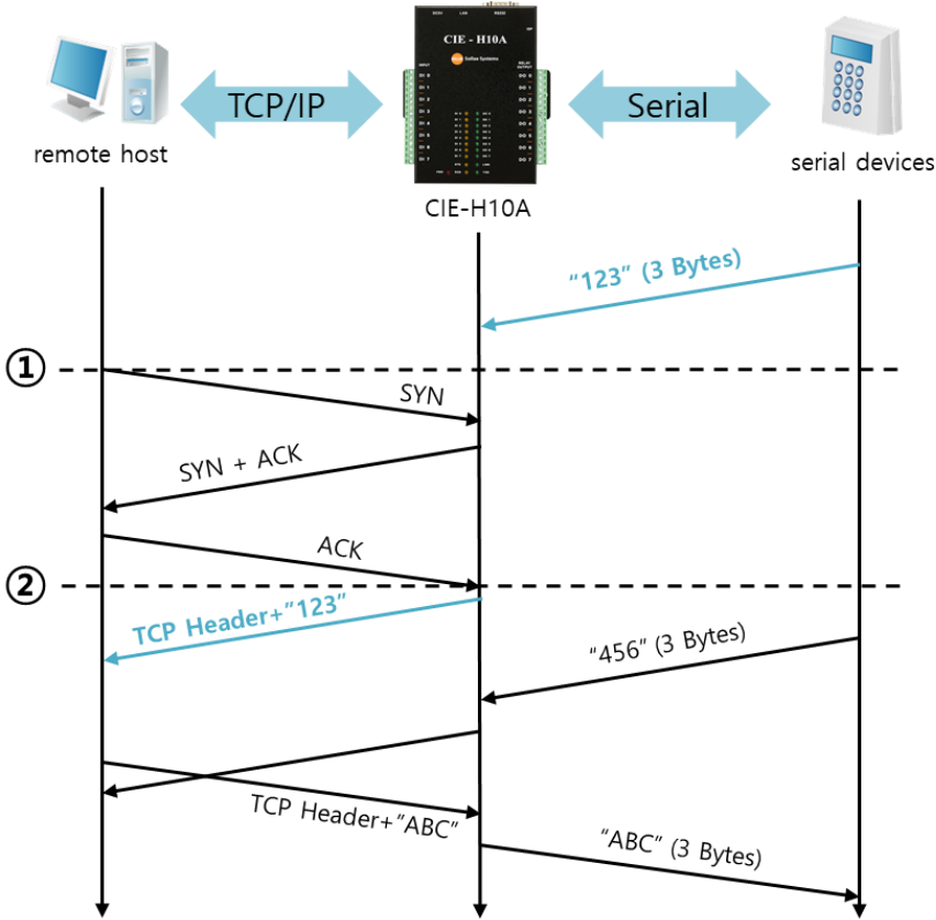
Figure 6-2 time chart
