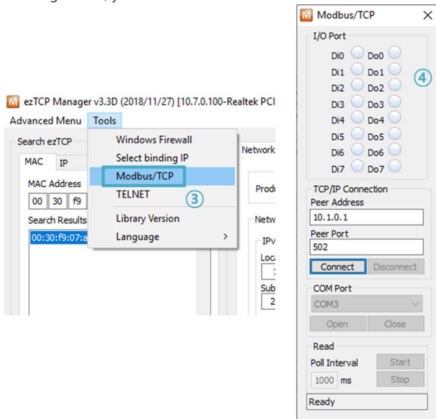
Figure 2-3 Modbus/TCP test program of the ezManager
