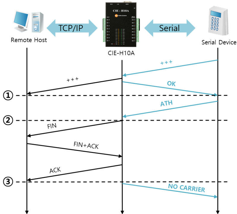
Figure 6-6 time chart
