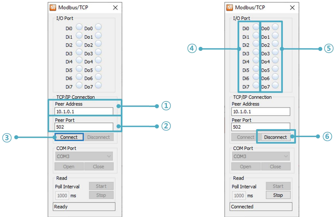
Figure 2-4 Modbus/TCP test
