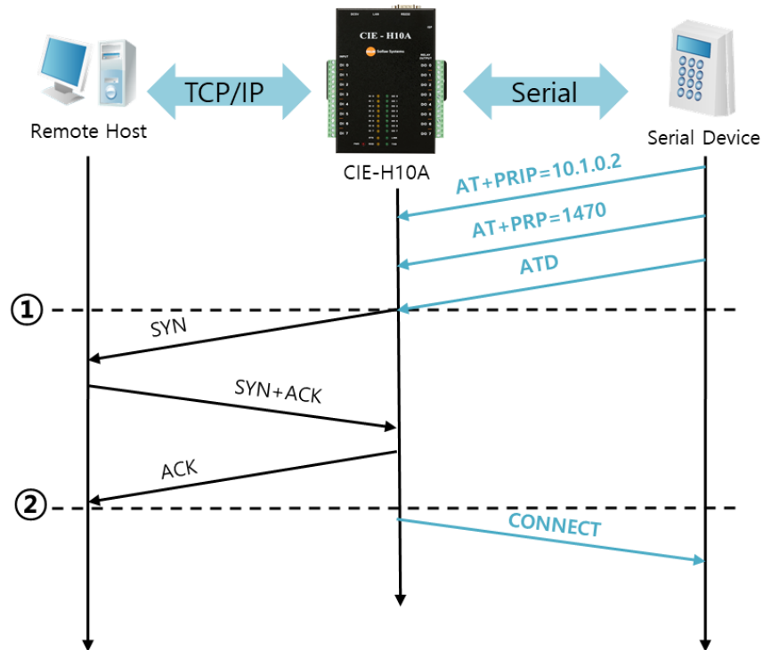
Figure 6-6 an active TCP connection
