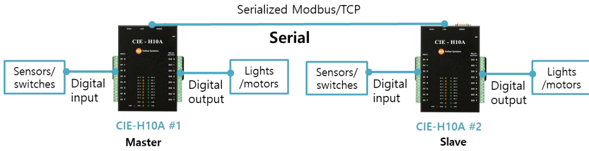
Figure 1-4 serial switch
