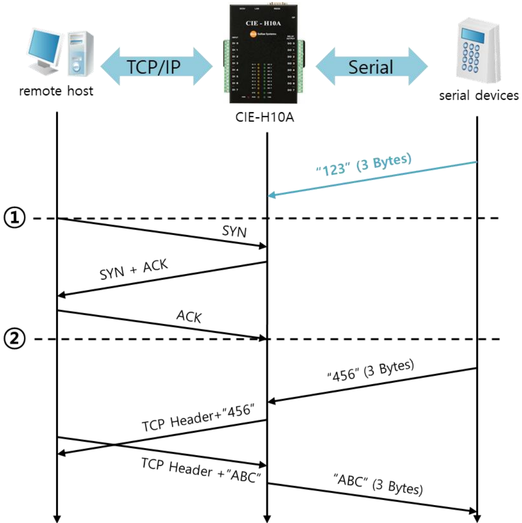
Figure 6-1 TCP server in the case [Event Byte] is set to 0
