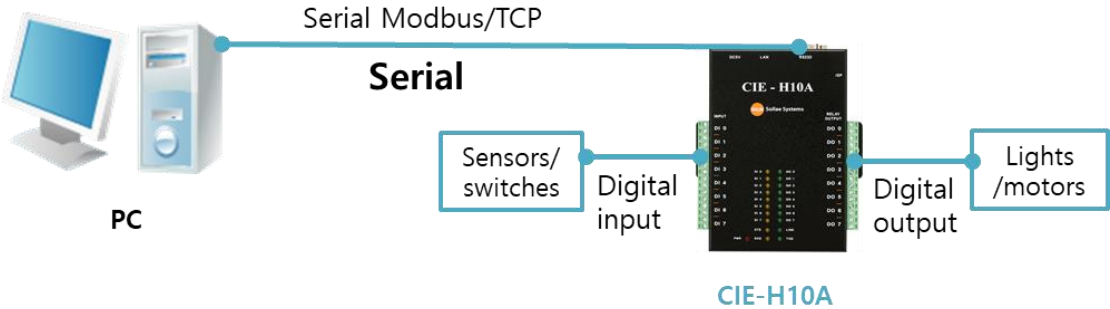
Figure 1-2 serialized Modbus/TCP
